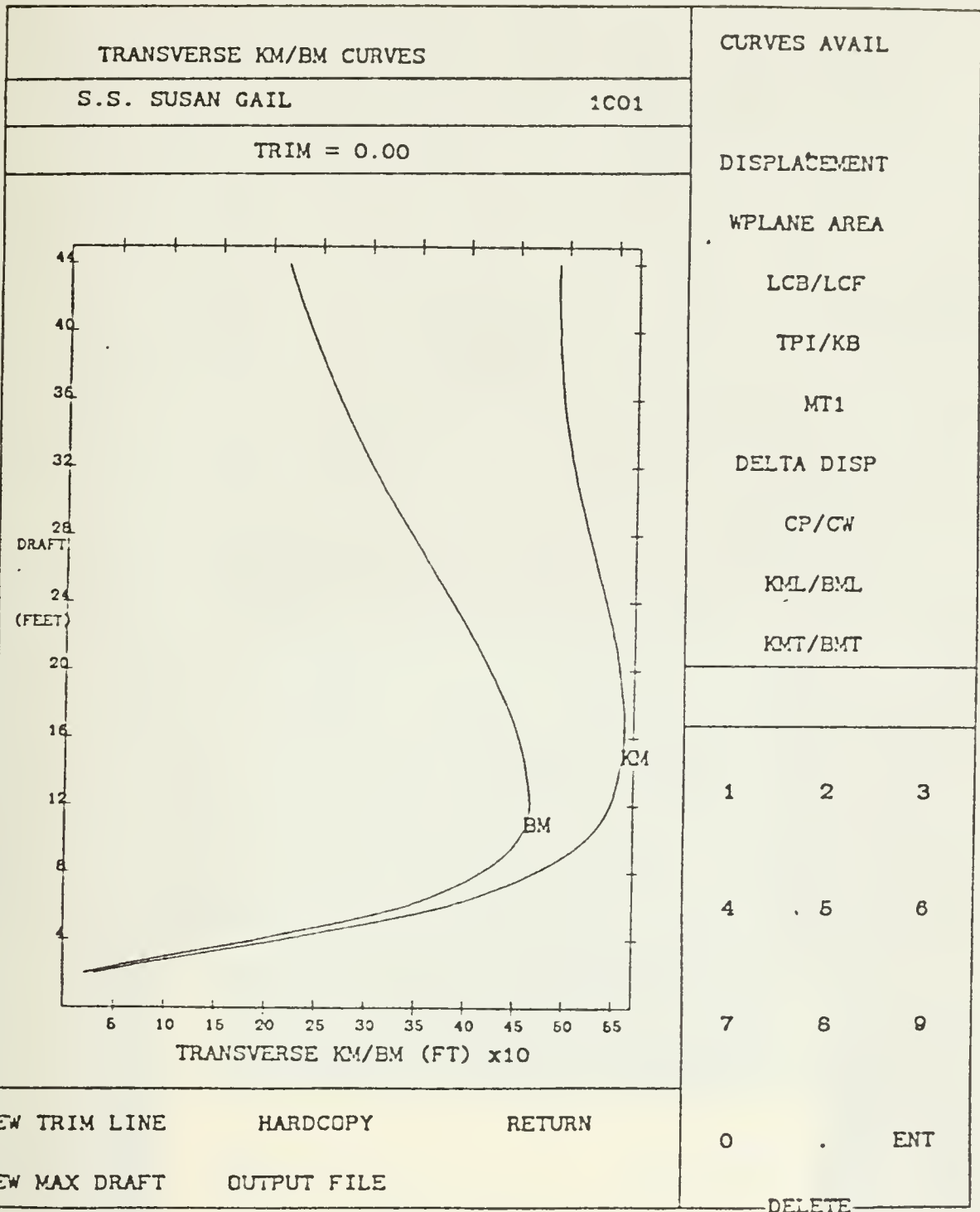
Figure H-12. Transverse KM/BM Curves
