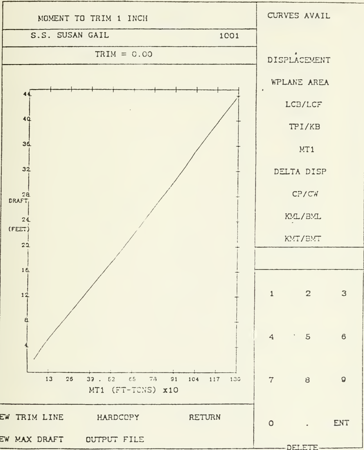
Figure H-8. Moment-to-Trim-One-Inch Curve
