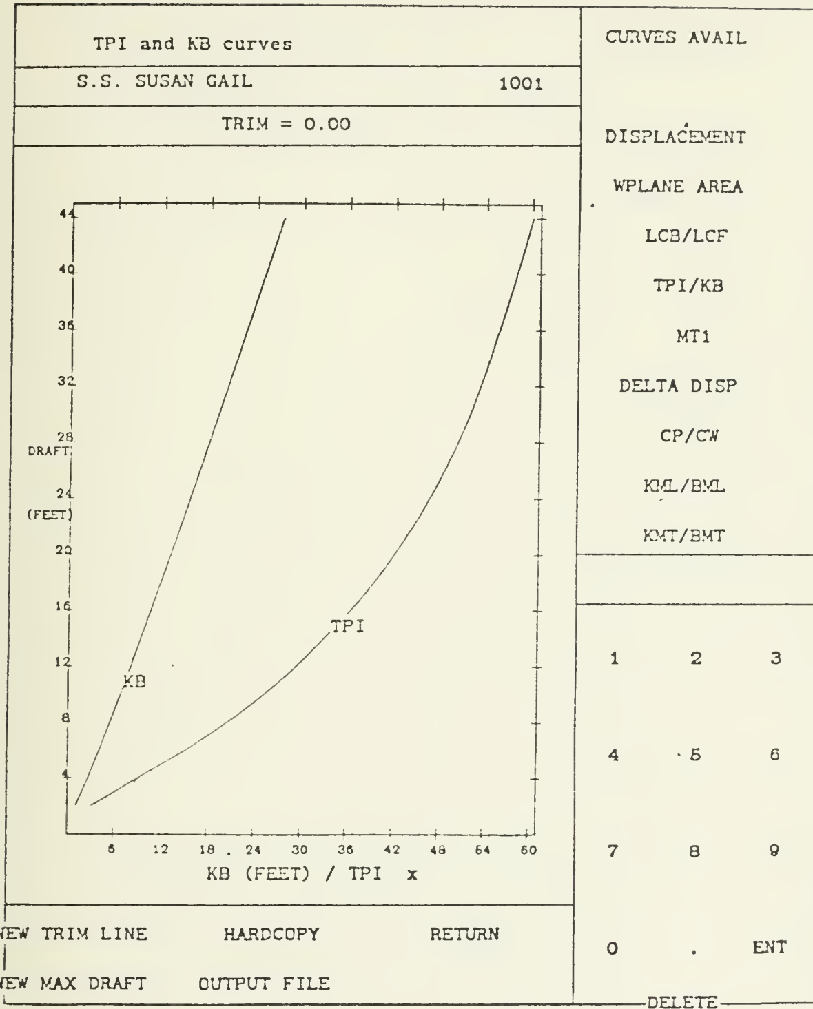
Figure H-7. TPI and KB Curves
