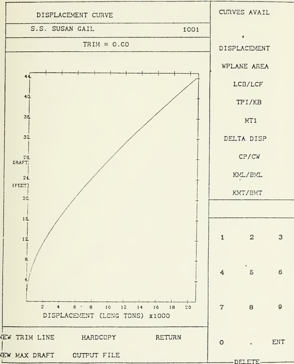
Figure H-4. Displacement Curve
