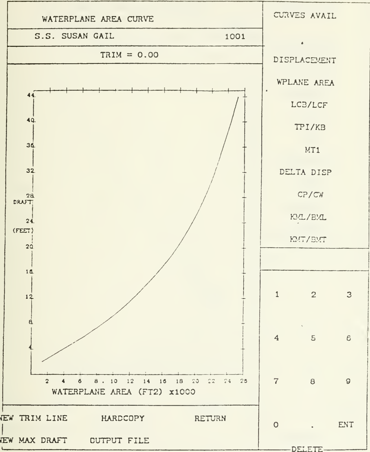
Figure H-5. Waterplane Area Curve
