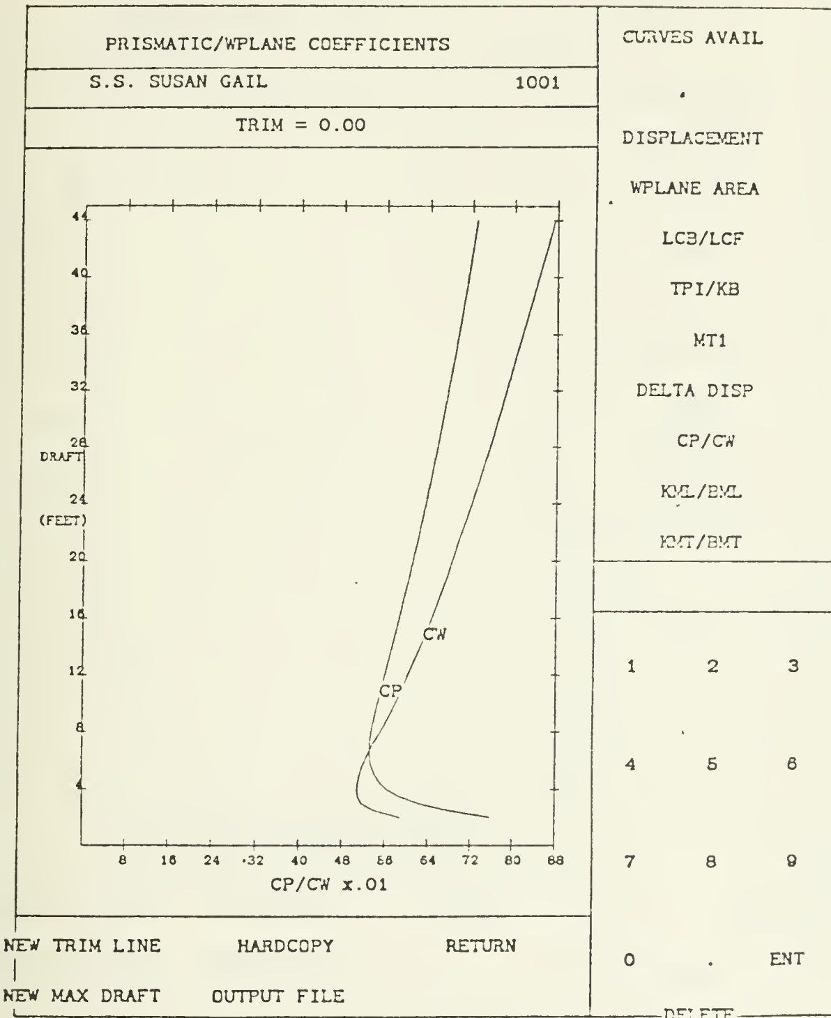
Figure H-10. Prismatic Coefficient/Waterplane Coefficient Curves.
